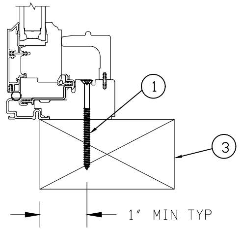
SILL
